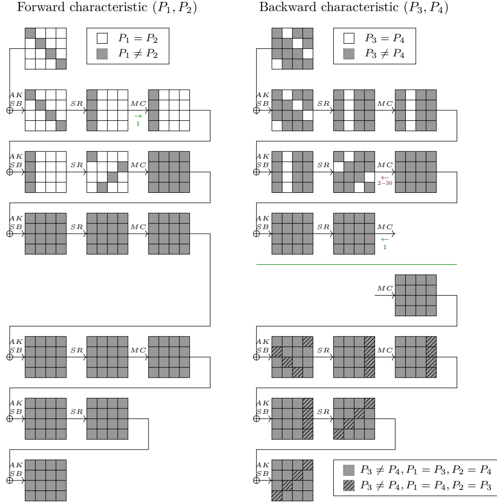
Figure 8: Fourth exchanged boomerang trail
