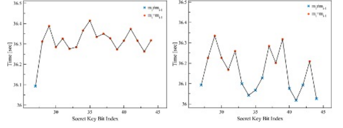
Fig. 14. The error detection (left) and correction (right) of bit index 33. The graphs for the additional five indexes that were corrected appear in Fig. ??
