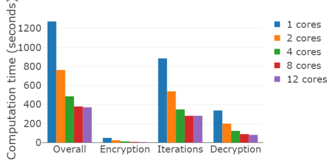
Figure 4. Computation time for increasing numbers of cores.
